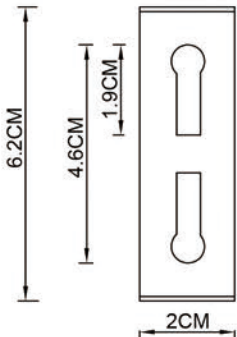
Hole position in the mounting bracket
